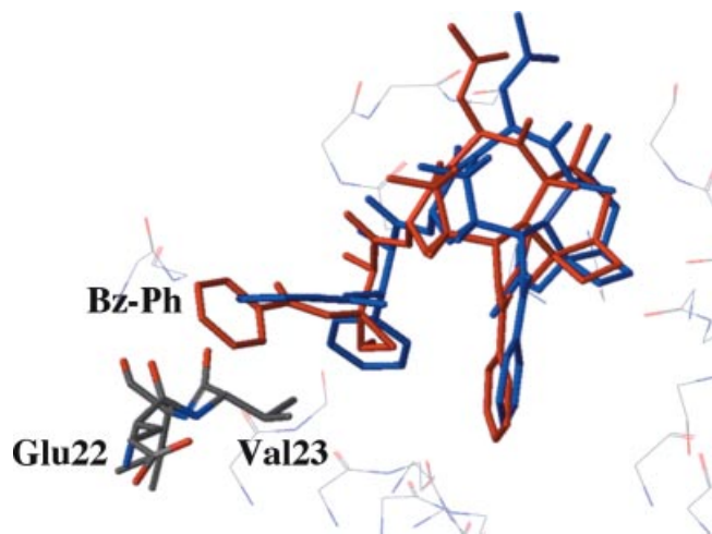
Figure 3. T-Taxol (blue) and cyclopropyl analog 3b (red) docked in the \beta -tubulin binding pocket and relaxed by low-temperature molecular dynamics. In response to internal steric strain in the concave region of the molecule, the molecular volume of the 3b expands by 2.0–2.2 Å from C-4 to C-3' and places the 3'-benzamido phenyl group (Bz-Ph) in unfavorable contact with tubulin's Glu22 and Val23 residues.
