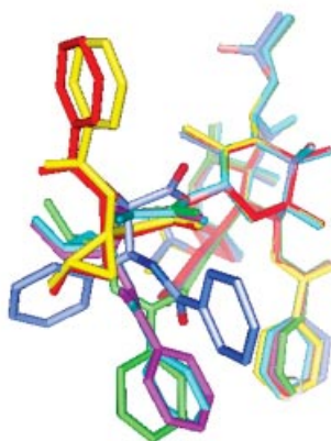
Figure 4. Five NAMFIS conformations of cyclopropane 3b in CDCl 3 (green, magenta, yellow, red, cyan) superimposed on the T-taxol conformer (blue) within the baccatin core. At the C-13 terminus, neither the phenyl rings nor the cyclopropane rings of the synthetic taxoids match the phenyl rings of taxol. Two methyl groups (yellow and red) fall near the middle of taxol's 3'-phenyl group.
