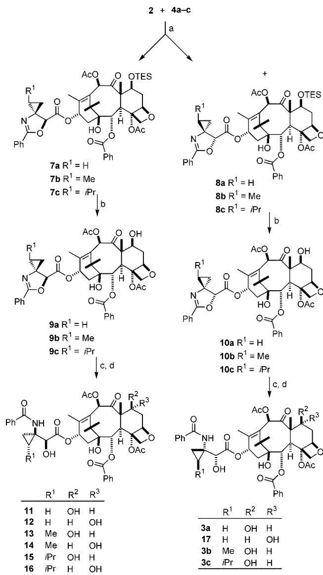
Scheme 2. Synthesis of C-3'-cyclopropanated taxol analogs. (a) DCC or EDC, 4-PP, toluene, room temp., 24 h, 85%; (b) HF/pyridine, THF, 0 °C to room temp., 24 h, 90%; (c) 0.1 N HCl/1,4-dioxane (1:1), 50 °C, 1–3 h, 85%; (d) 0.1 N NaHCO 3 /1,4-dioxane (1:1), room temp., 6–24 h, 80%.
