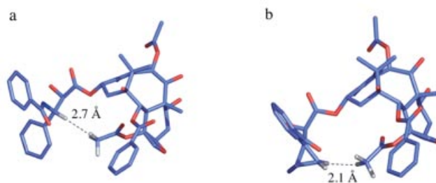
Figure 2. T-Taxol conformations illustrating the potential for steric congestion between the 4-OAc methyl group and the C-3' center. a) The H...H distances between 3'-H and the 4-OAc methyl group in T-taxol are above the sum of the van der Waals radii ( 2.7 \text{ \AA} ); b) cyclopropyl H atoms as in 3b engage in severe van der Waals contacts with the 4-OAc methyl group ( 2.1 \text{ \AA} ).
