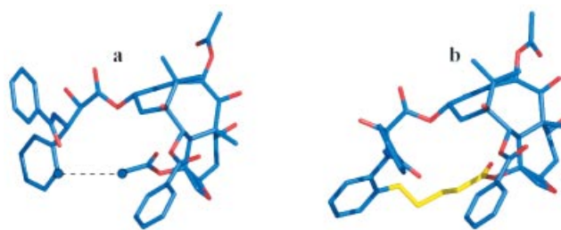
Figure 1. Taxol analog conformations at the \beta -tubulin binding site. a) T-Taxol conformer illustrating the close contact between the 4-OAc methyl group and the ortho position of the phenyl group at C-3'; b) A C-4-C-3'-bridged taxane with activity equivalent to parent taxol.
