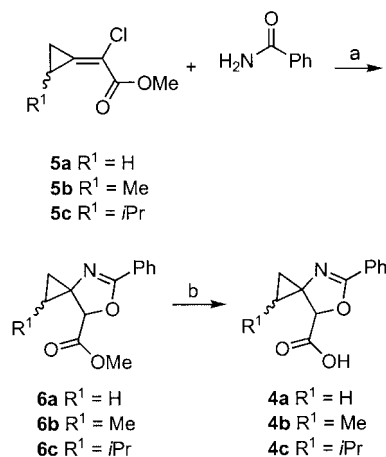
Scheme 1. Synthesis of cyclopropanes 4a–4c . (a) NaH, MeCN, 0 °C to room temp., 20 h, 16–60%; (b) NaOH, THF, room temp., 20 h, 58–100%.
