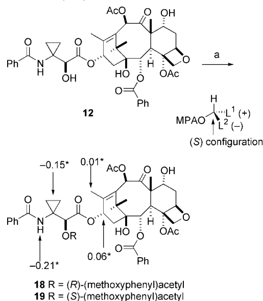
Scheme 3. Determination of the absolute configuration of 12 . (a) ( R )- \alpha -Methoxyphenylacetic acid or ( S )- \alpha -methoxyphenylacetic acid, EDC, DMAP, CH 2 Cl 2 , room temp., 24 h, 85%. * \Delta\delta^{RS} = \delta^R(18) - \delta^S(19) .
